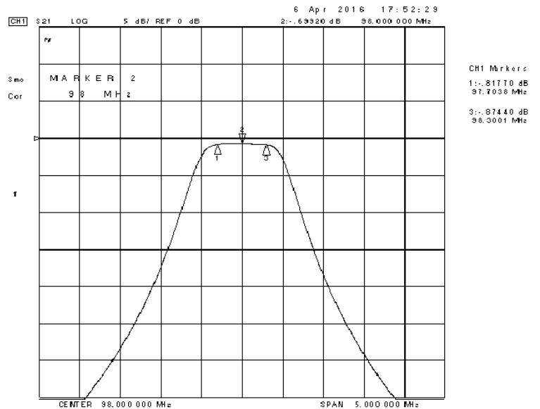
INSERTION LOSS
