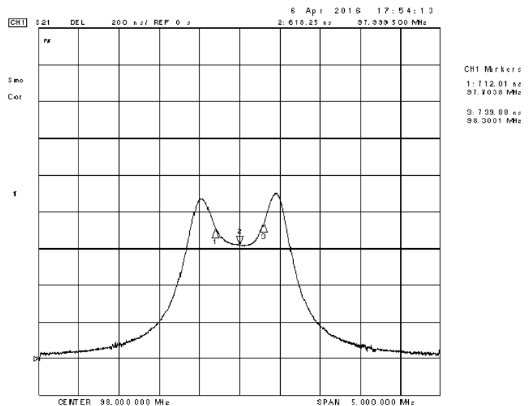
GROUP DELAY
